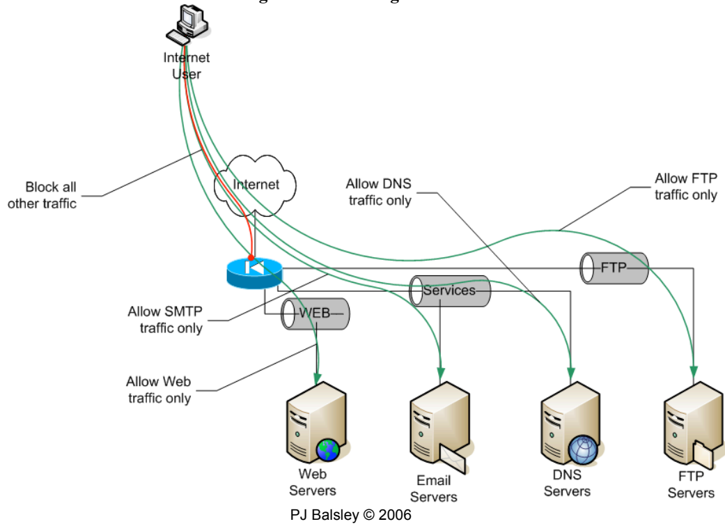
Figure 6 - Incoming Traffic
