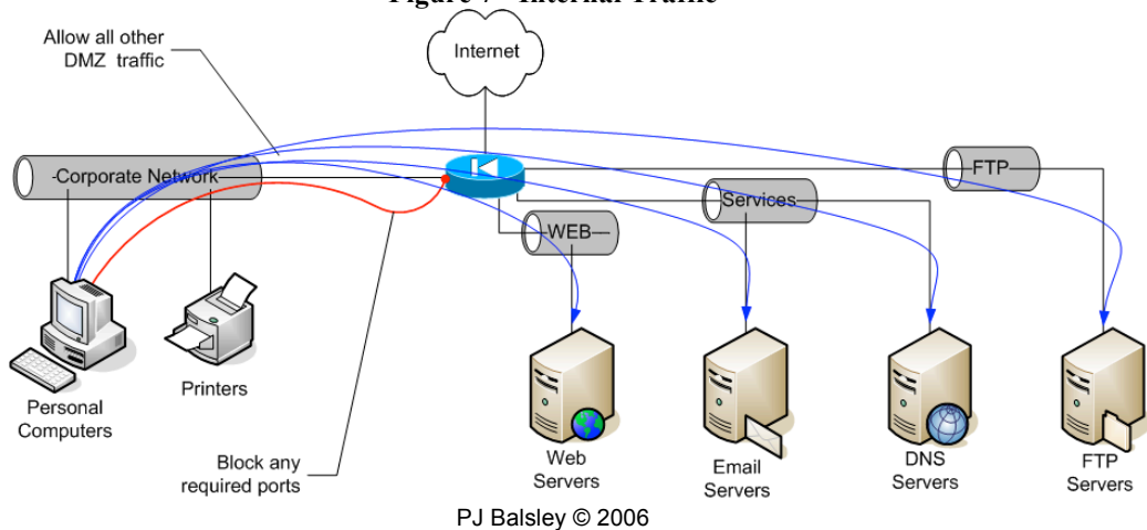
Figure 7 - Internal Traffic
